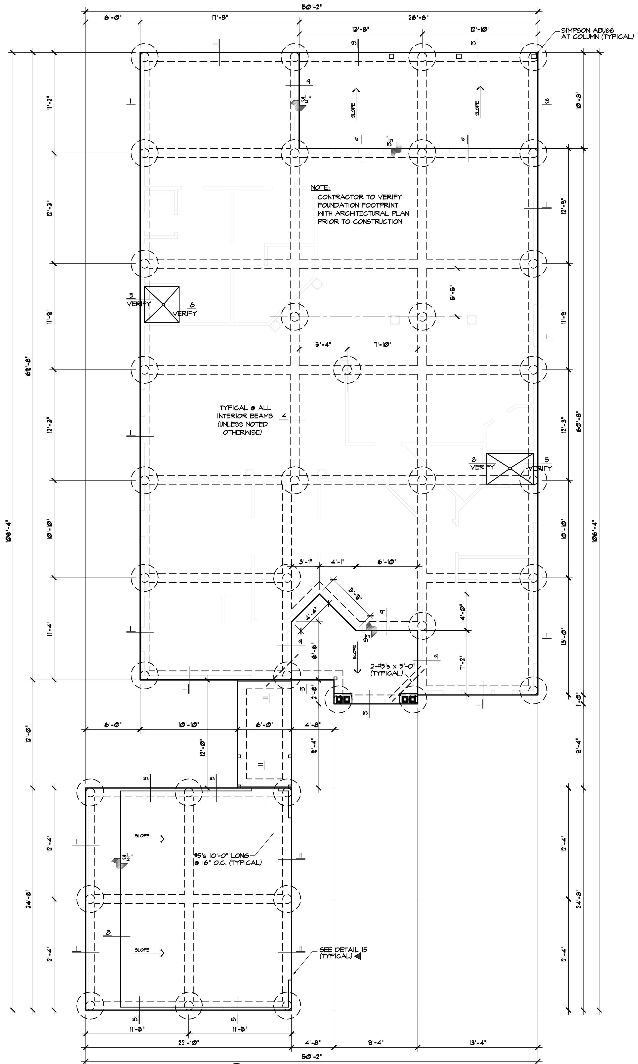
1 FOUNDATION PLAN SCALE: 3/16"=1'-0"
